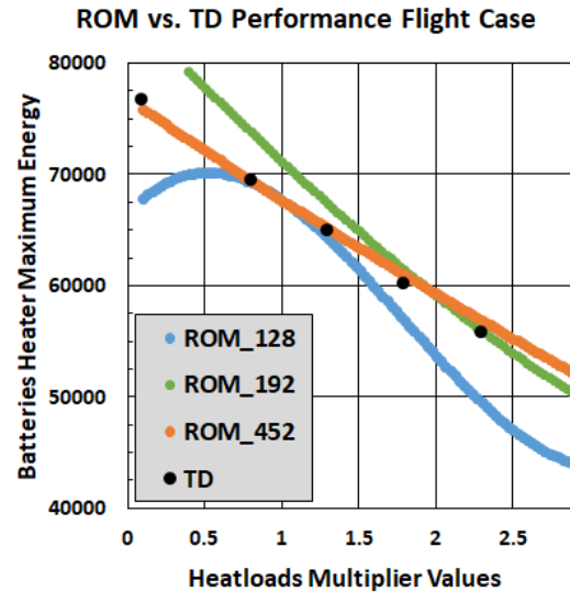
Figure 3. ROM vs. Thermal Desktop® Performance for the Flight case.
