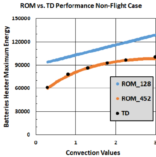
Figure 4. ROM vs. Thermal Desktop® Performance for the Non-Flight case.
