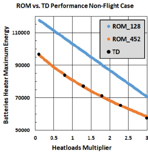
Figure 4. ROM vs. Thermal Desktop® Performance for the Non-Flight case.
